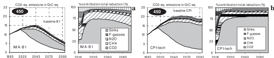
Figure 2. Contribution of greenhouse gases in total emission reductions for the emission pathways for a stabilization at 450ppm CO 2 -eq. concentration of the IMA-B1 (a) and CPI+tech scenario (b).
